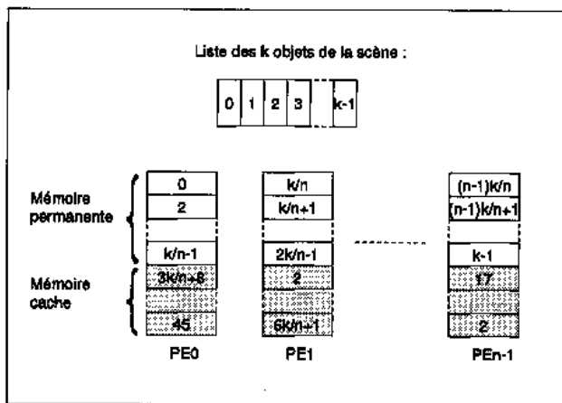
Figure 53 Organisation de la mémoire
