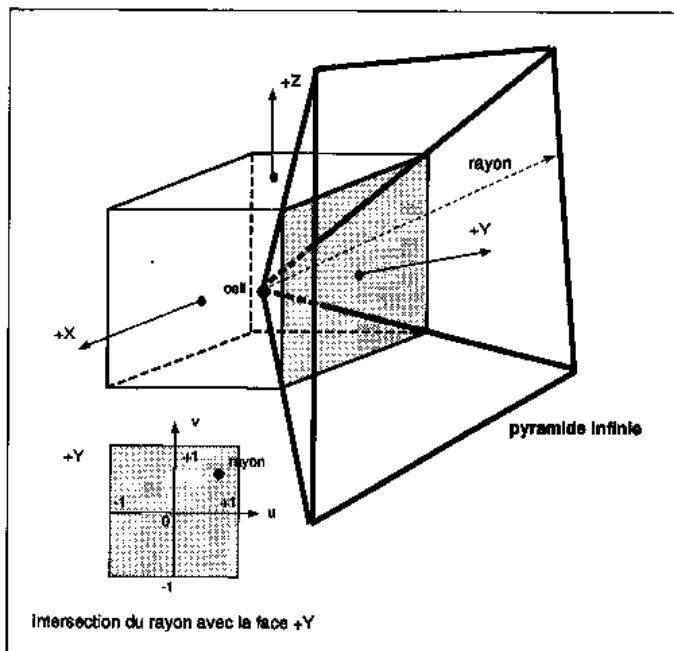
Figure 20 Le cube de direction
