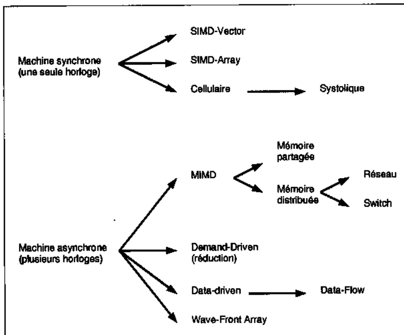
Figure 24 La classification de MIMESIS
