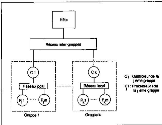
Figure 33 Architecture hiérarchique
