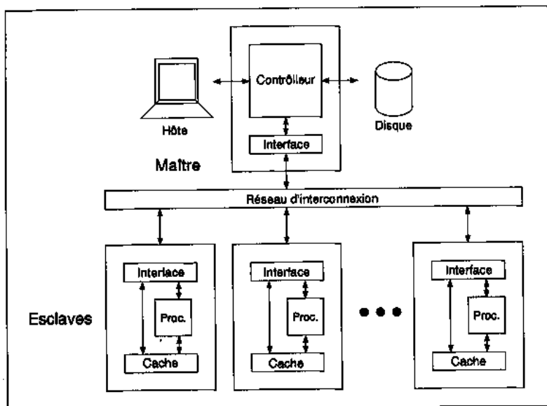
Figure 35 Architecture maître-esclaves
