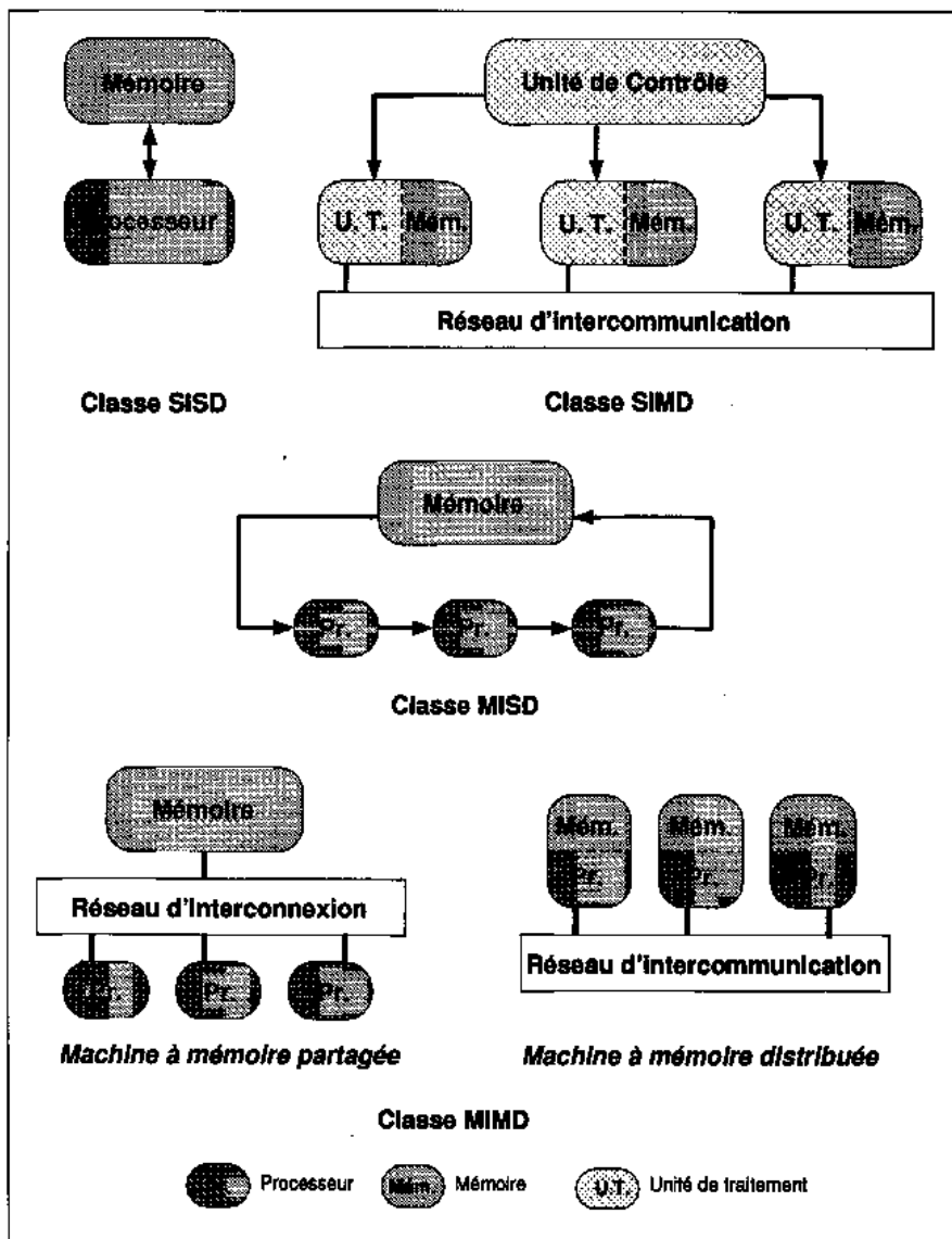
Figure 22 La classification de Flynn
