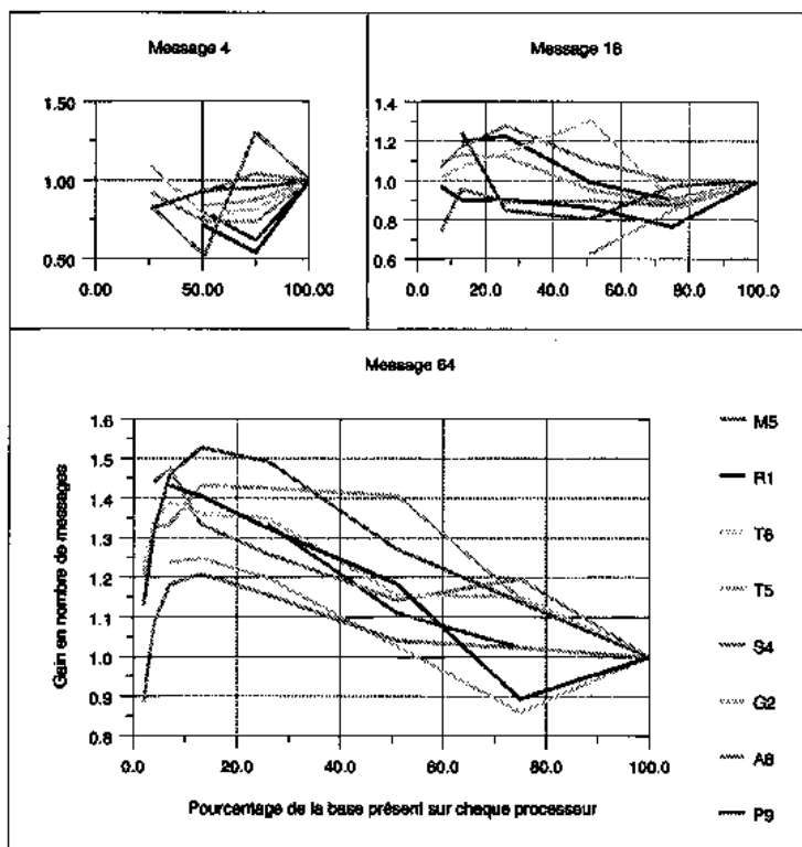
Figure 84 Gain en messages
